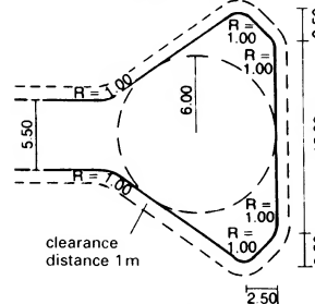
7 As 6
